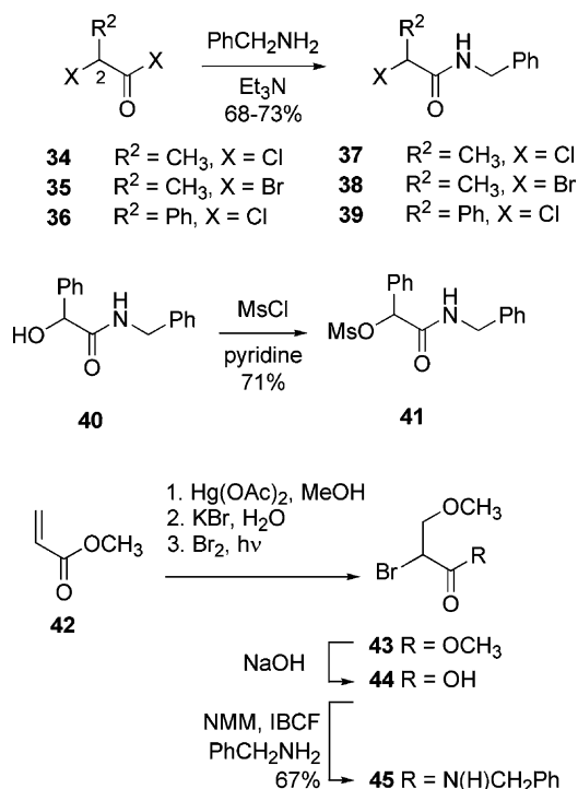
Scheme 2. Synthesis of N -benzyl-2-substituted amides.
