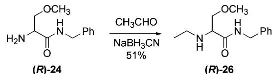
Scheme 3. Synthesis of ( R )- N -benzyl-2-ethylamino-3-methoxypropionamide.
