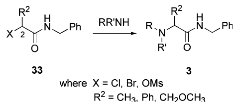
Scheme 1. General synthetic route to AAA.
