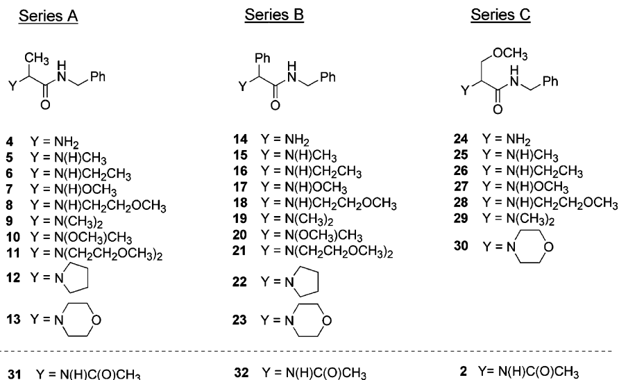
Figure 1. Sites of AAA modification.
