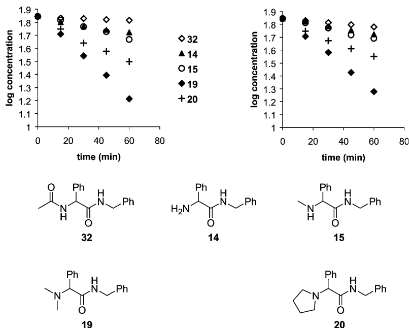
Figure 3. In vitro metabolism rate of substrate consumption of C(2) phenyl AAA. Incubations were performed with 1 mg microsomal protein, 1 mM NADPH, and 100 \mu M substrate at room temperature for 60 min.
